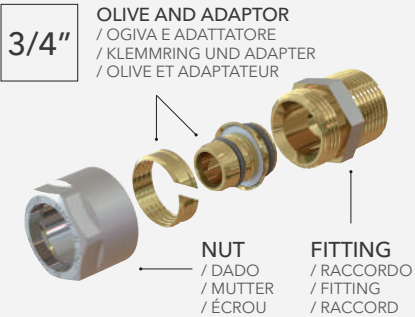
KIT 3/4"
