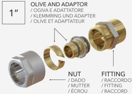
KIT 1"
