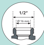
PRE-ASSEMBLED TAIL
